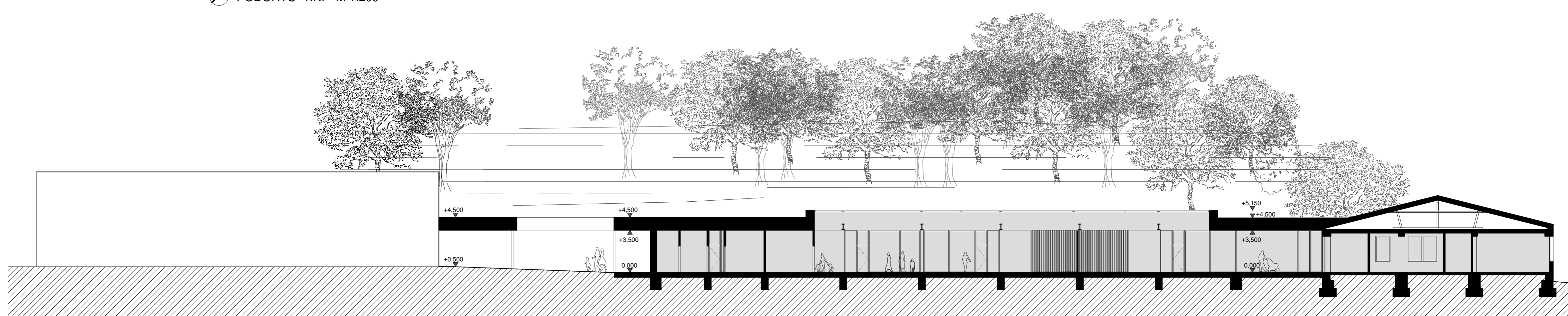
REZ A - A M 1:200
